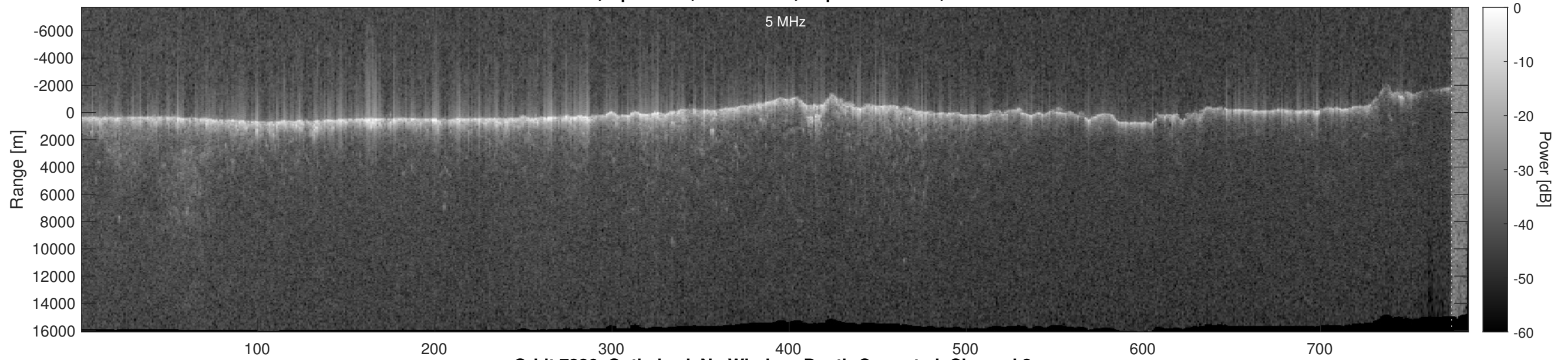
Orbit 7326, Optimized, No Window, Depth-Corrected, Channel 2
