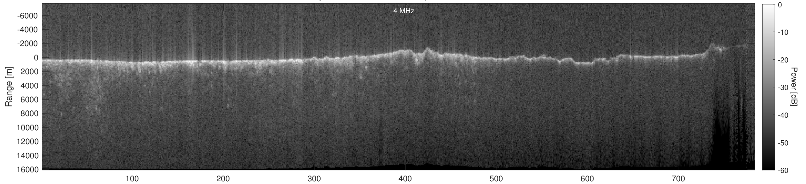
Orbit 7326, Depth-Corrected Cluttergram
