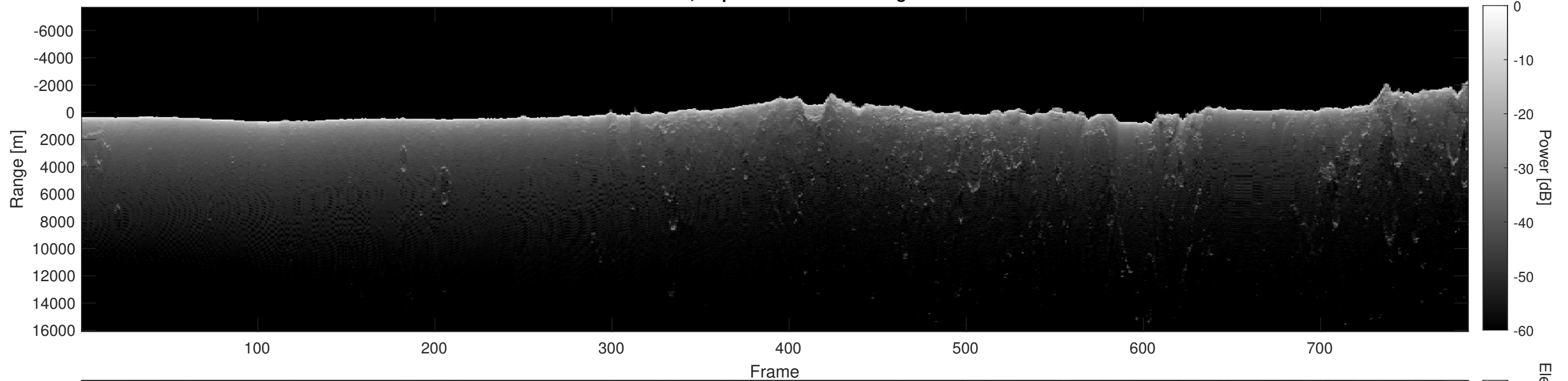
Orbit 7326, Depth-Corrected Cluttergram
