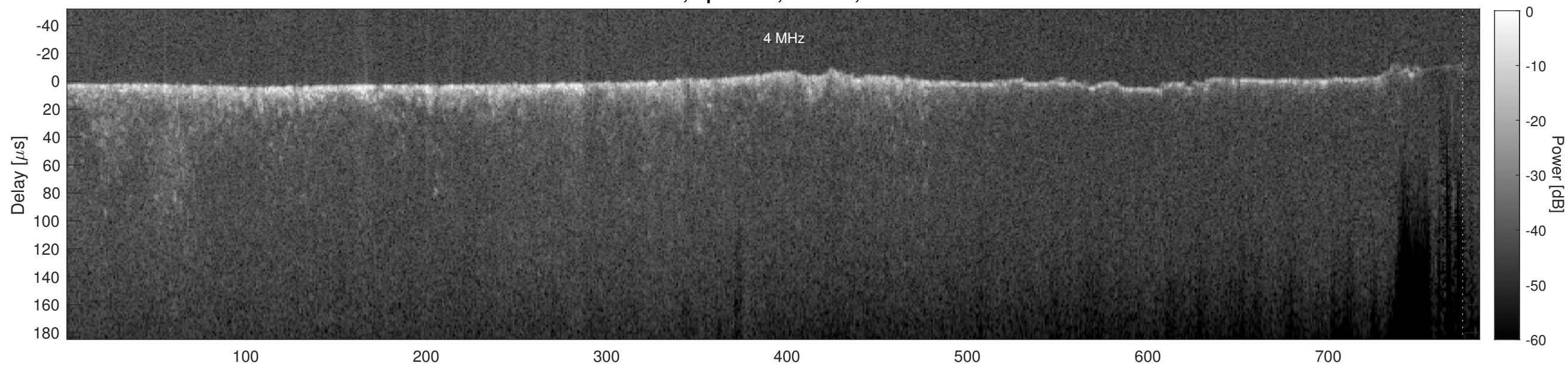
Orbit 7326, Cluttergram
