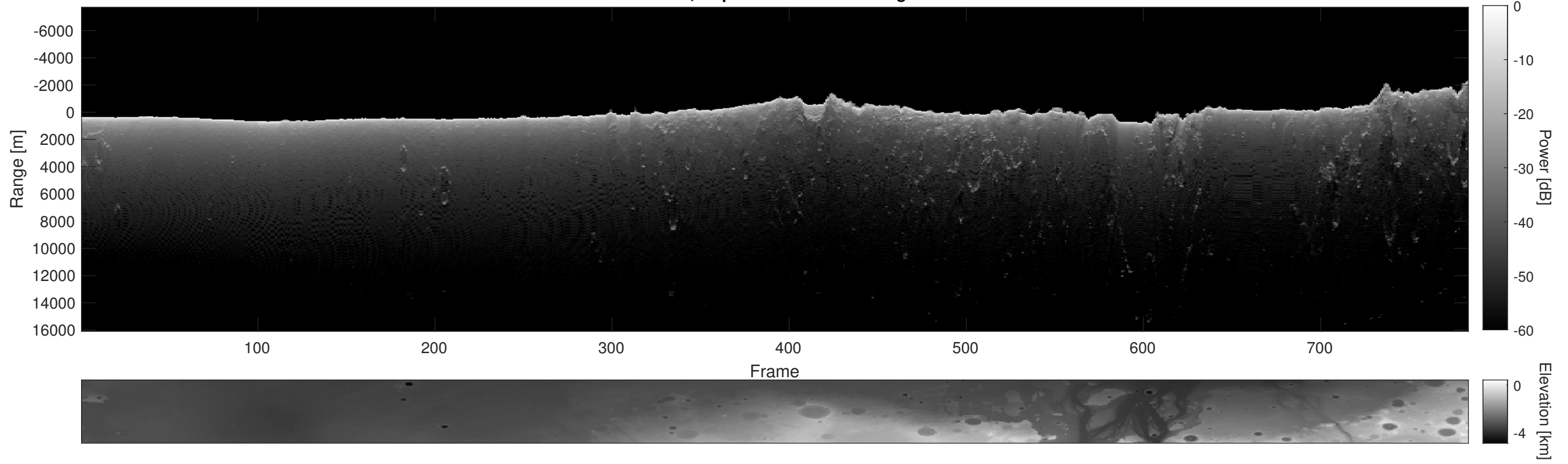
Orbit 7326, Depth-Corrected Cluttergram
