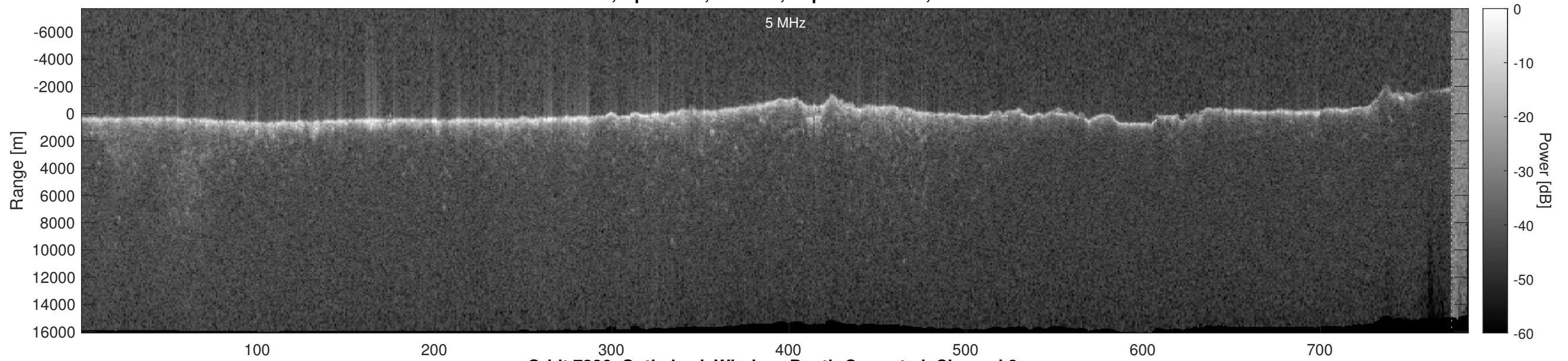
Orbit 7326, Optimized, Window, Depth-Corrected, Channel 2
