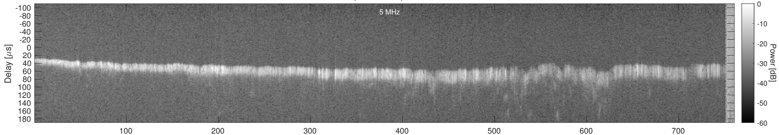
Orbit 7332, Window, Channel 1, Chapman
