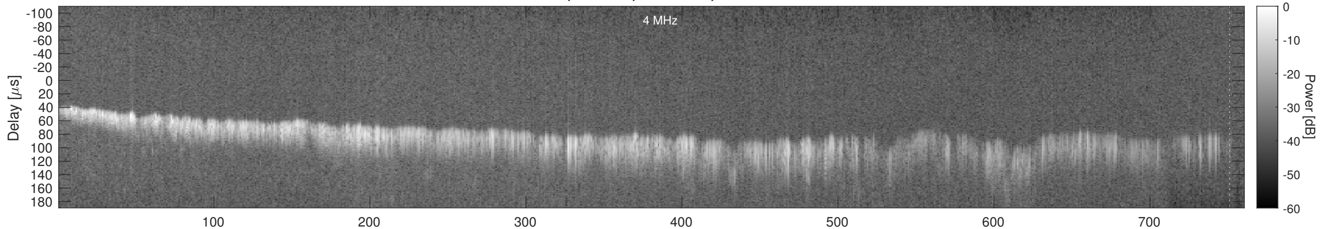
Orbit 7332, Window, Channel 2, Chapman
