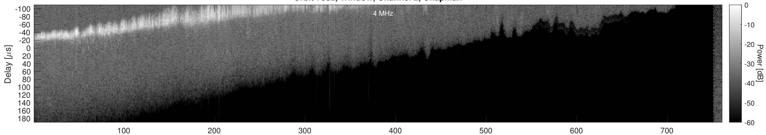
Orbit 7332, Window, Channel 2, Optimized
