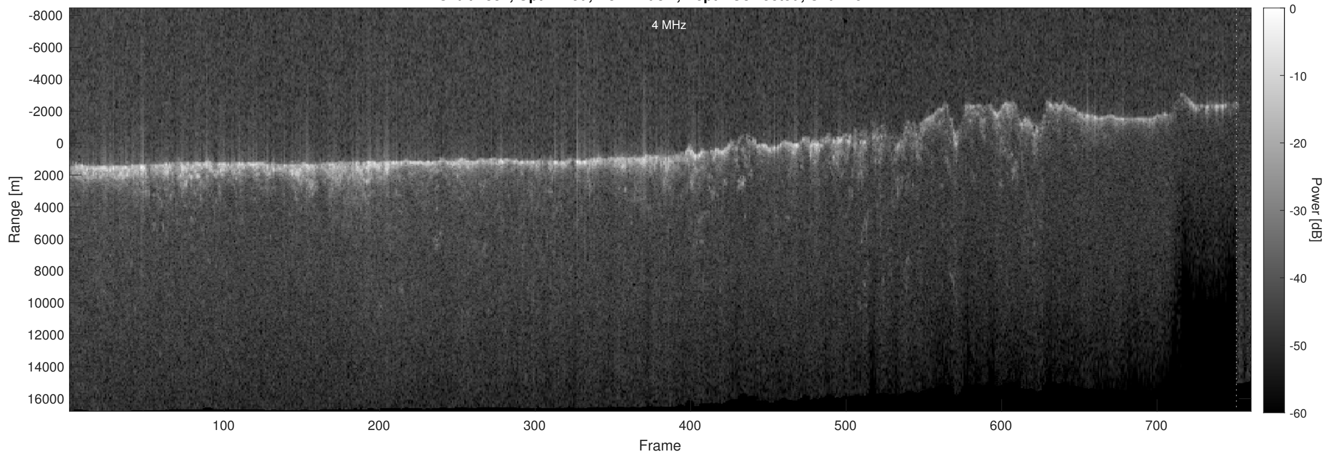
Orbit 7332, Optimized, No Window, Depth-Corrected, Channel 2
