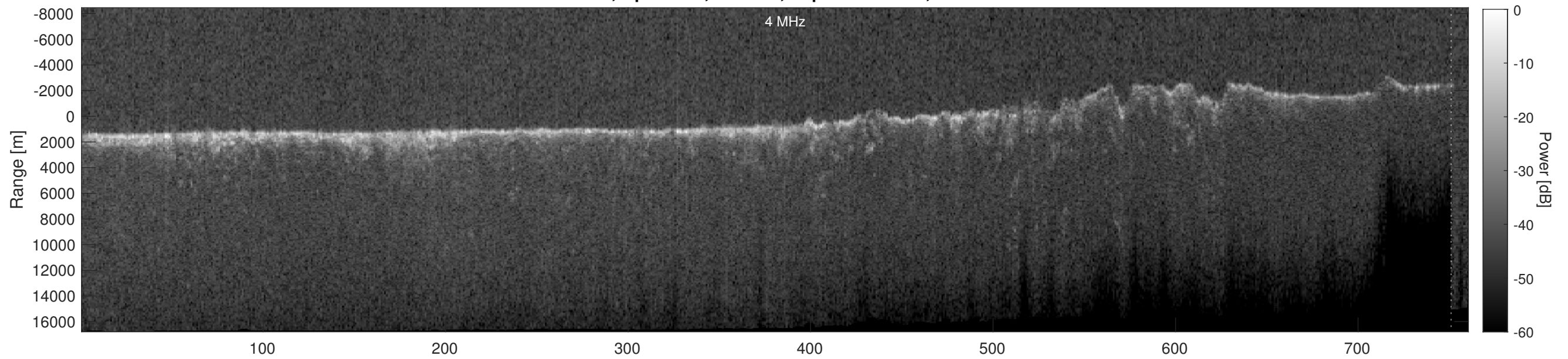
Orbit 7332, Depth-Corrected Cluttergram
