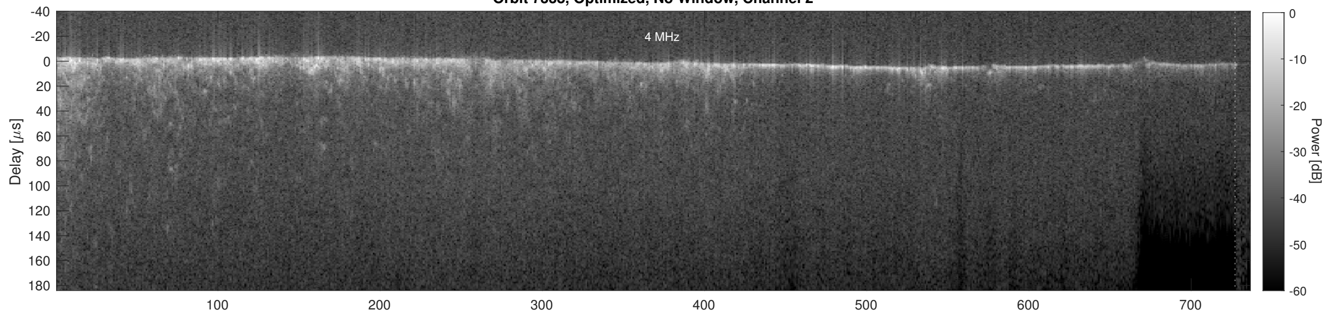
Orbit 7338, Cluttergram
