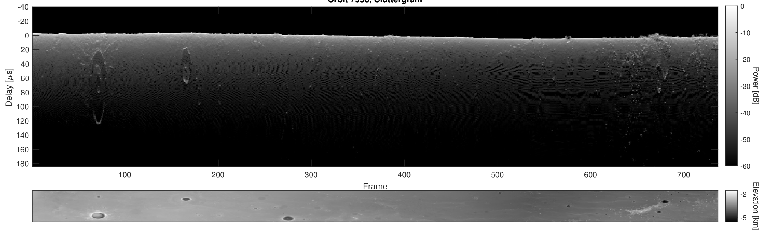
Orbit 7338, Cluttergram
