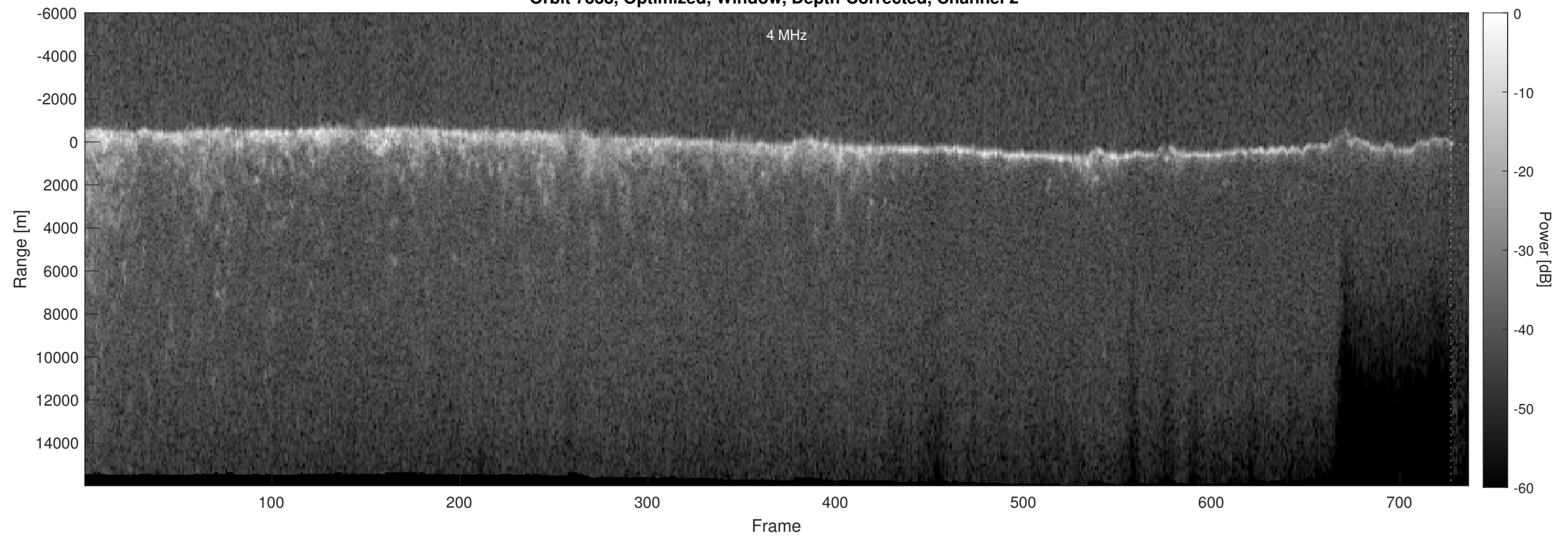
Orbit 7338, Optimized, Window, Depth-Corrected, Channel 2
