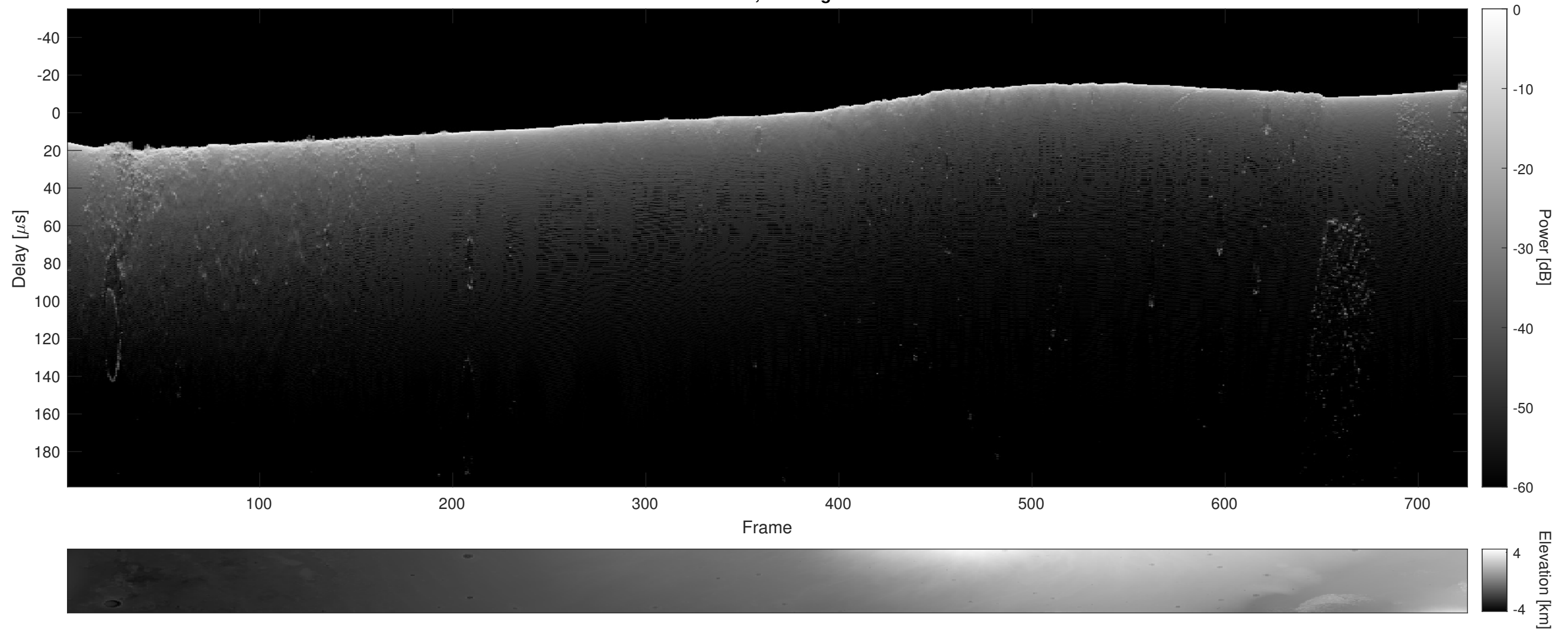
Orbit 7341, Cluttergram
