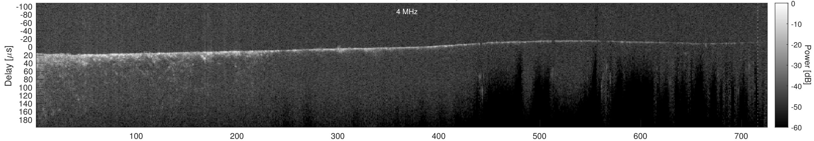
Orbit 7341, Cluttergram
