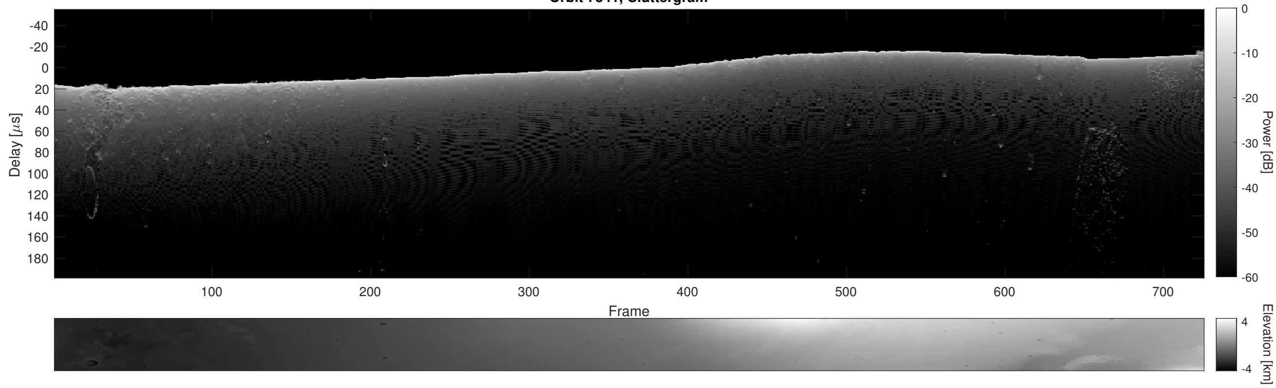
Orbit 7341, Cluttergram
