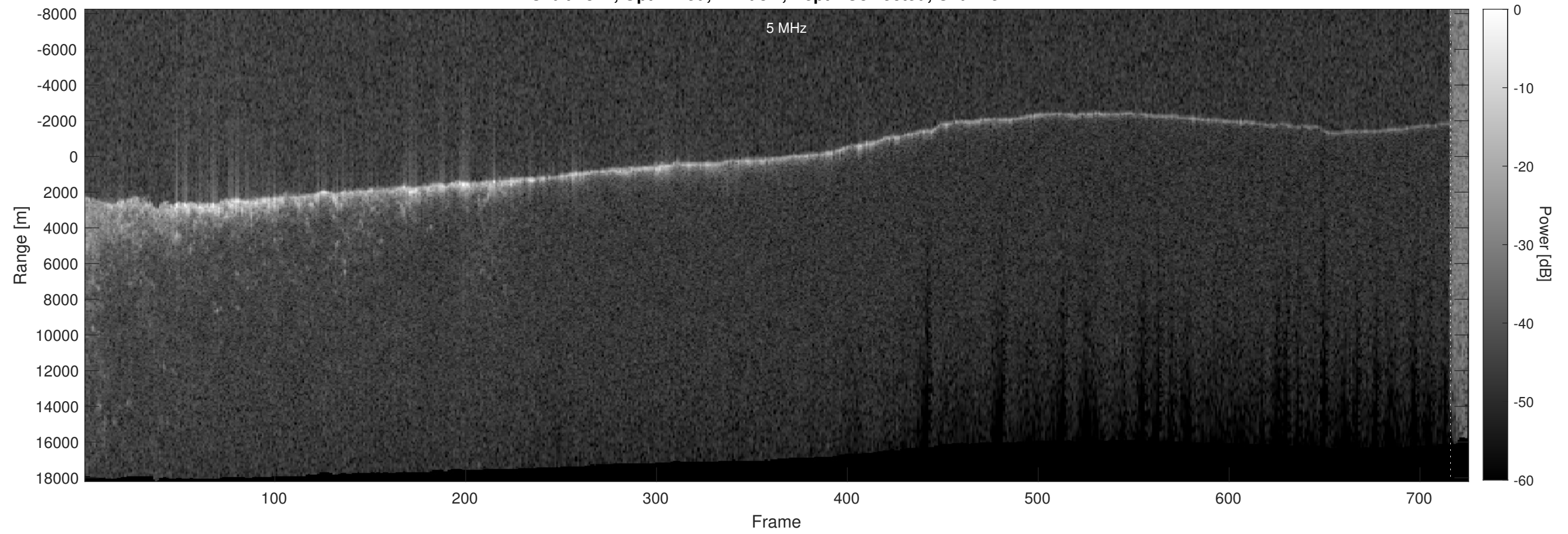
Orbit 7341, Optimized, Window, Depth-Corrected, Channel 2
