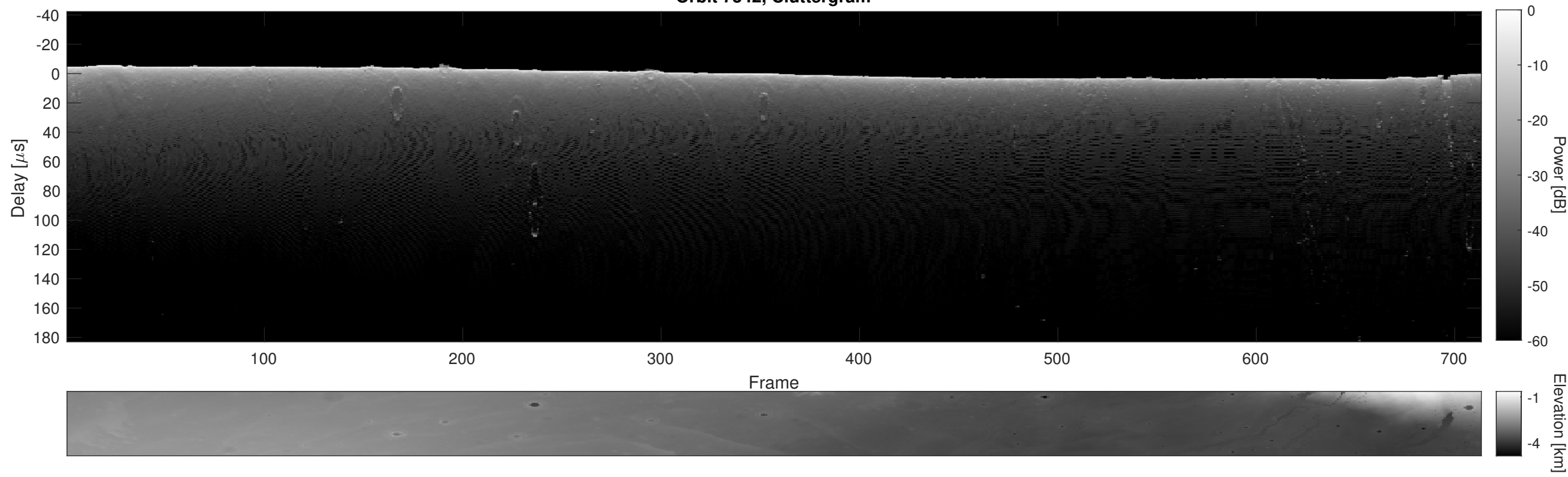
Orbit 7342, Cluttergram
