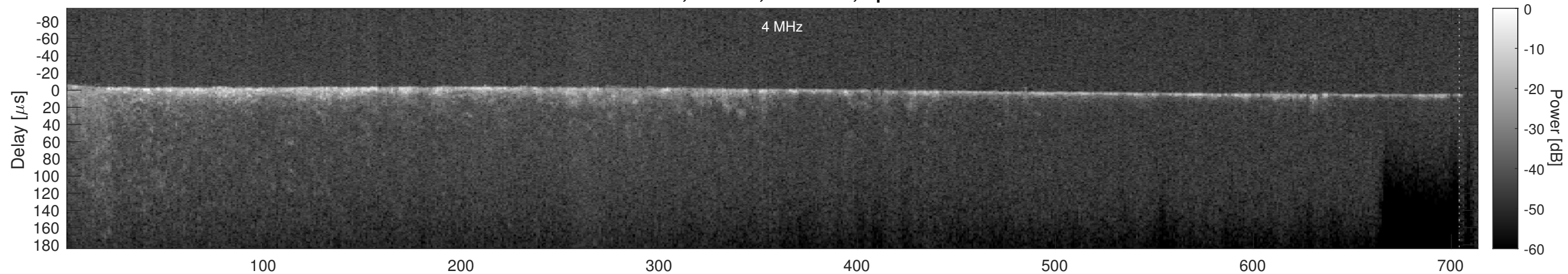
Orbit 7345, Cluttergram
