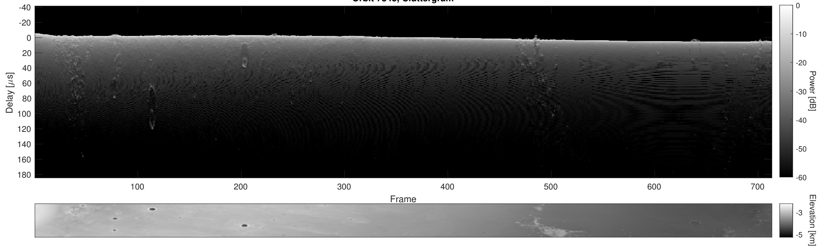
Orbit 7345, Cluttergram
