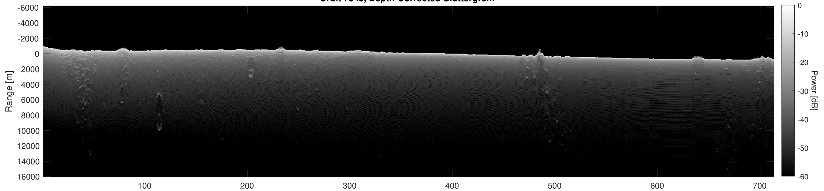
Orbit 7345, Depth-Corrected Cluttergram
