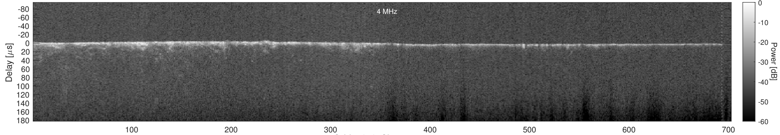
Orbit 7346, Cluttergram
