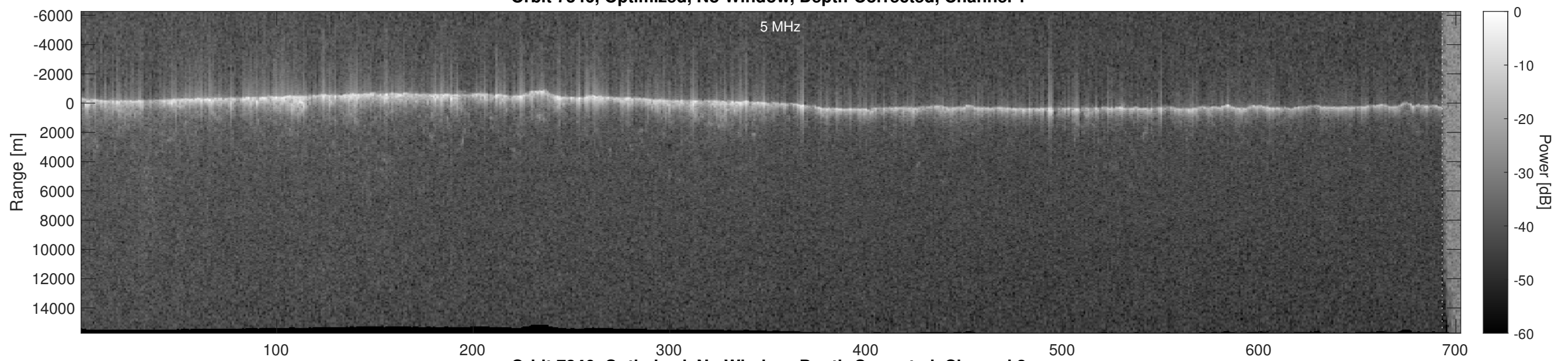
Orbit 7346, Optimized, No Window, Depth-Corrected, Channel 2
