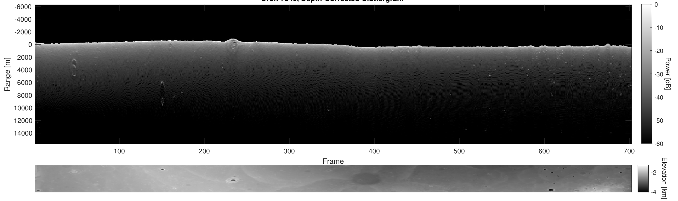
Orbit 7346, Depth-Corrected Cluttergram
