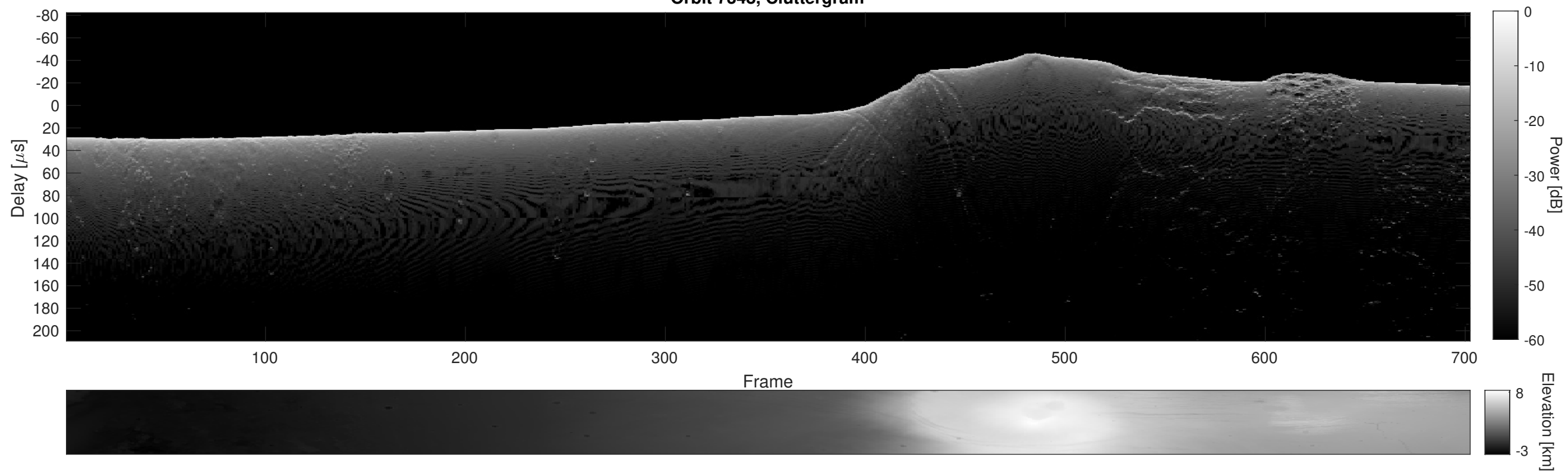
Orbit 7348, Cluttergram
