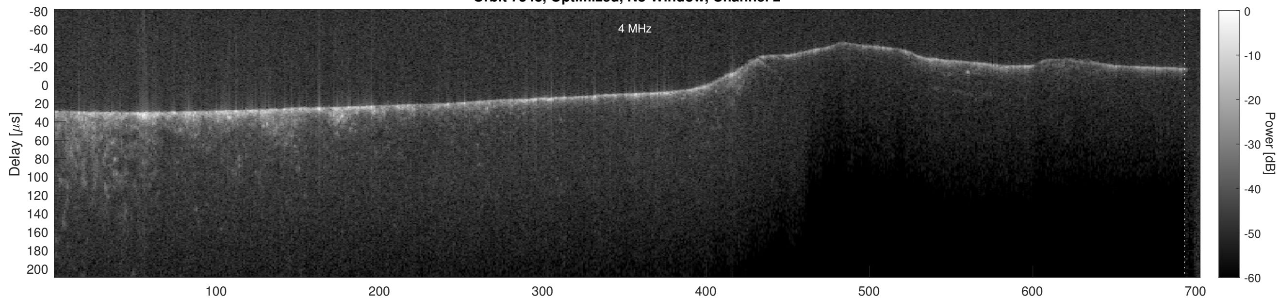
Orbit 7348, Cluttergram
