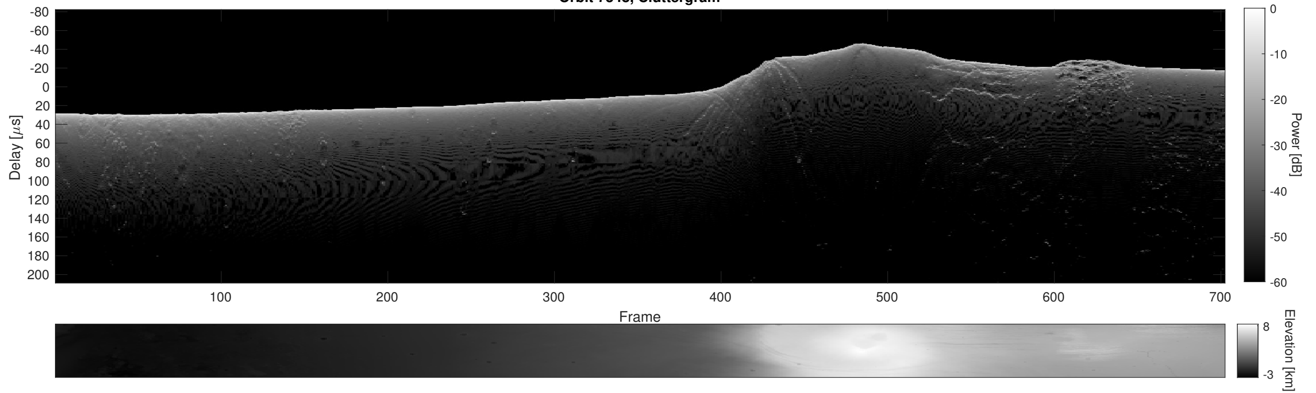
Orbit 7348, Cluttergram
