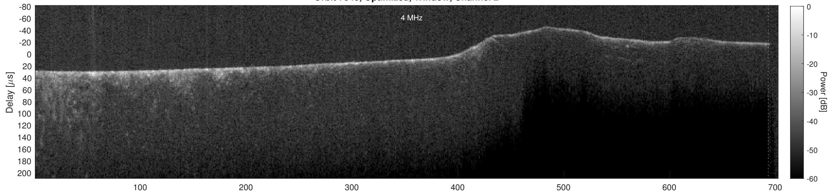
Orbit 7348, Cluttergram
