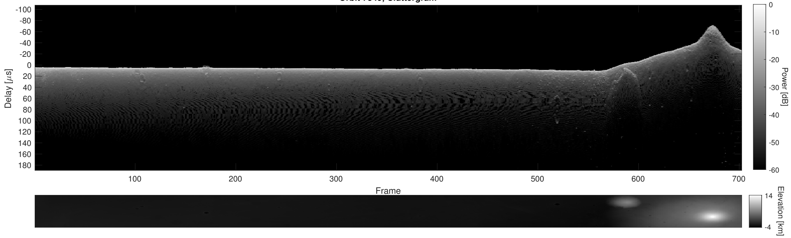
Orbit 7349, Cluttergram
