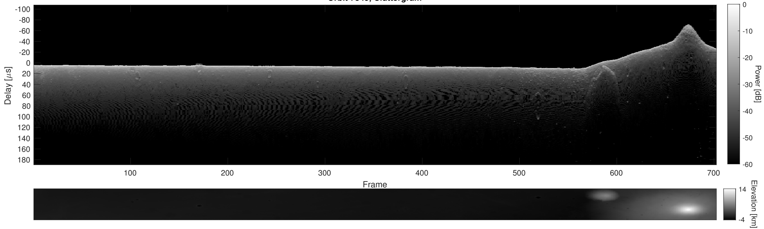
Orbit 7349, Cluttergram
