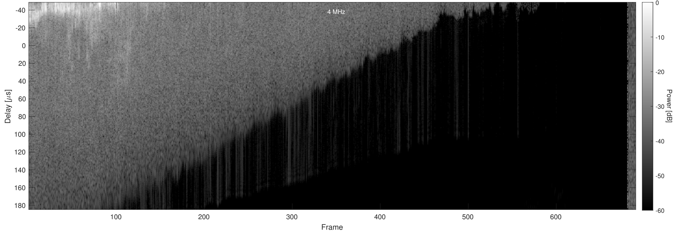
Orbit 7351, Chapman, No Window, Channel 2
