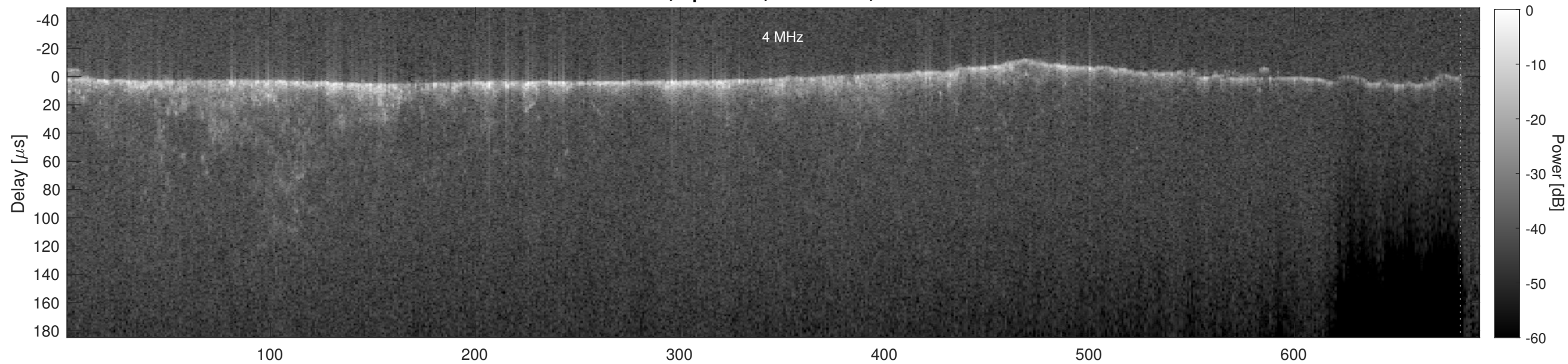
Orbit 7351, Cluttergram
