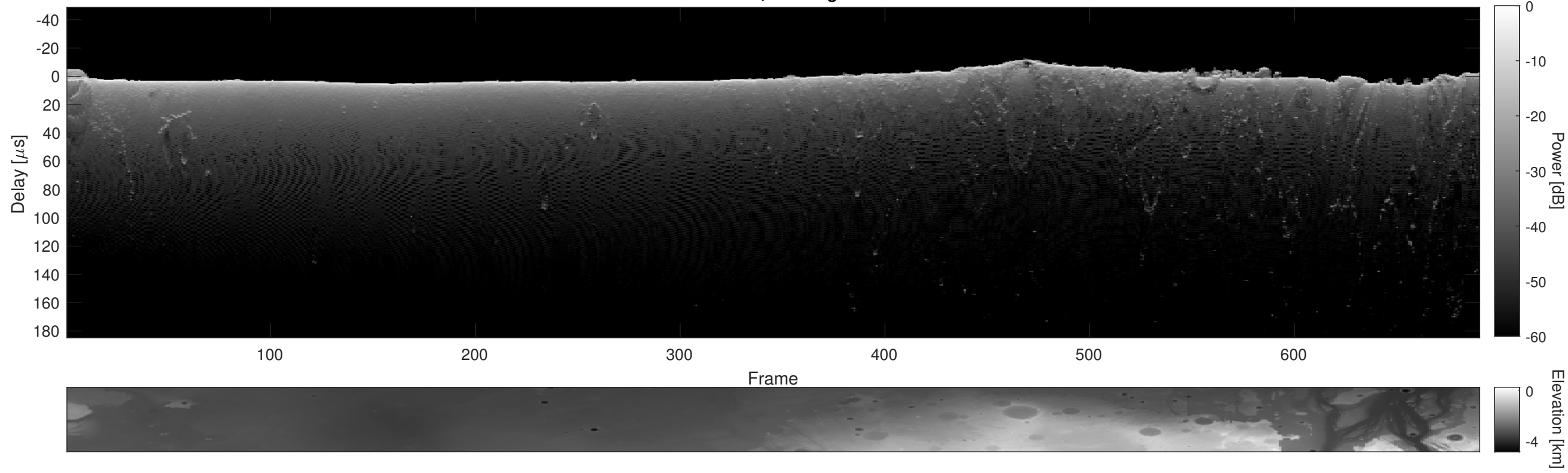
Orbit 7351, Cluttergram
