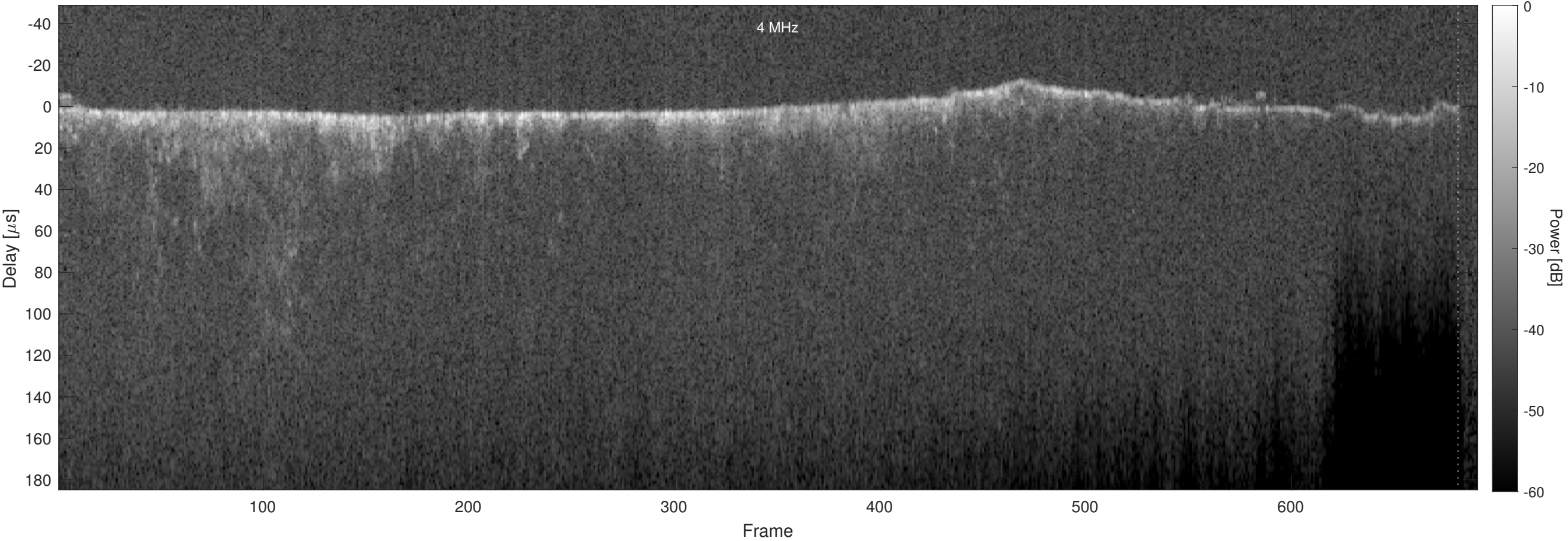
Orbit 7351, Optimized, Window, Channel 2
