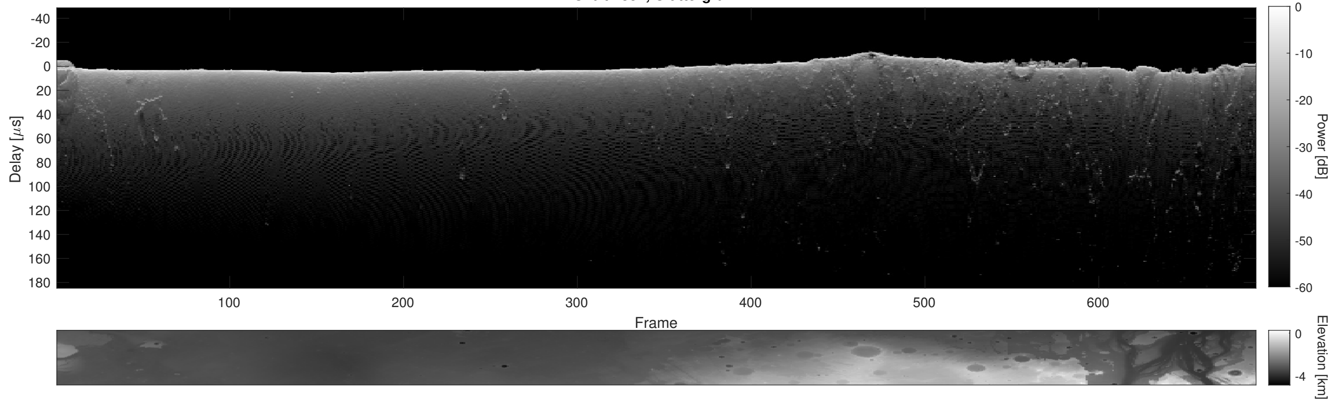
Orbit 7351, Cluttergram
