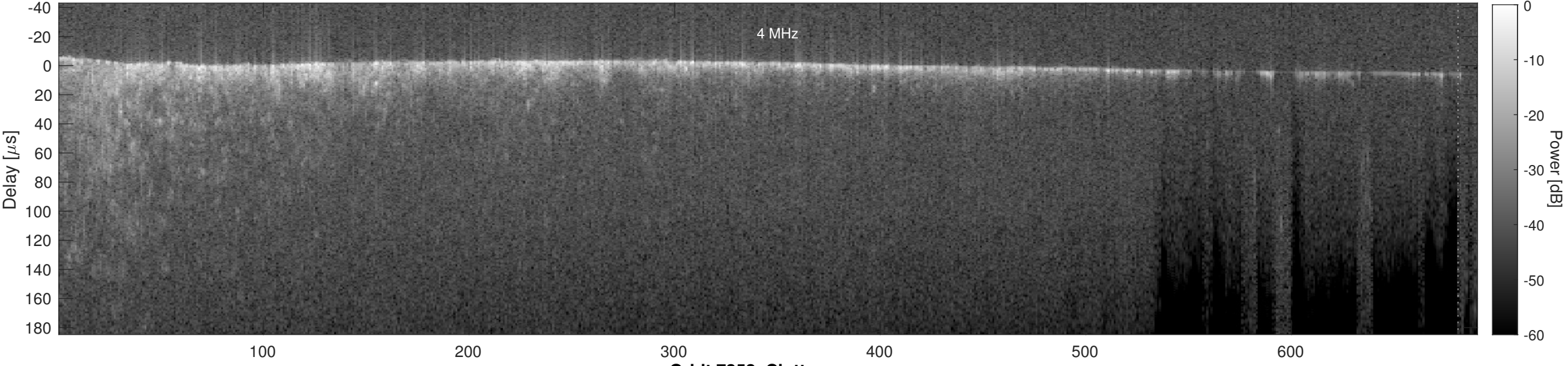
Orbit 7352, Cluttergram
