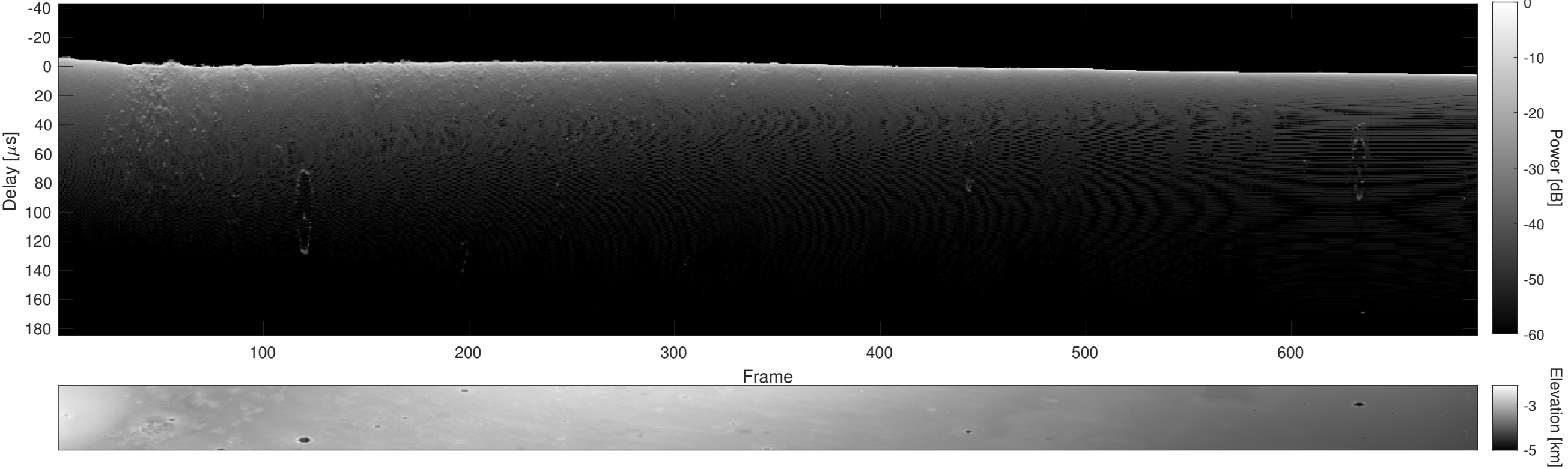
Orbit 7352, Cluttergram
