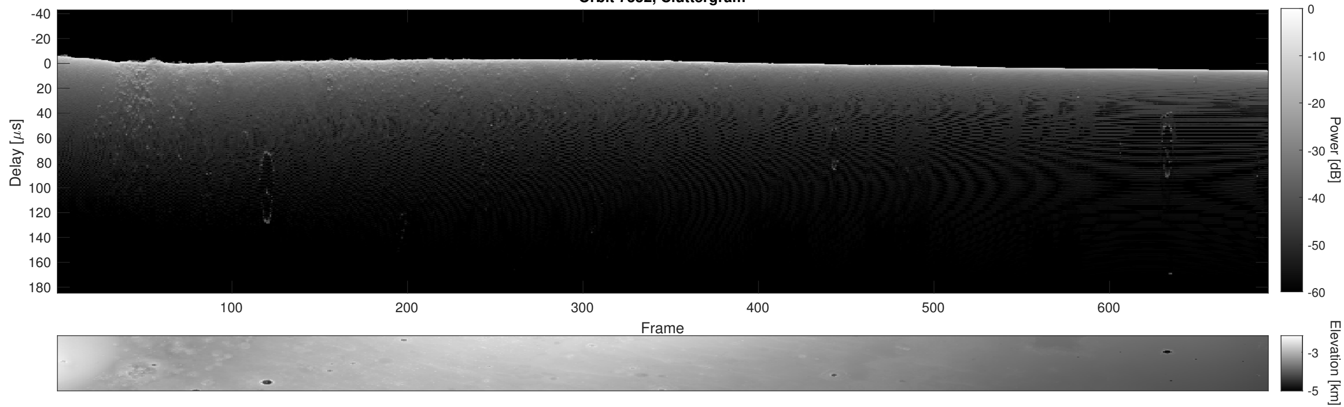
Orbit 7352, Cluttergram
