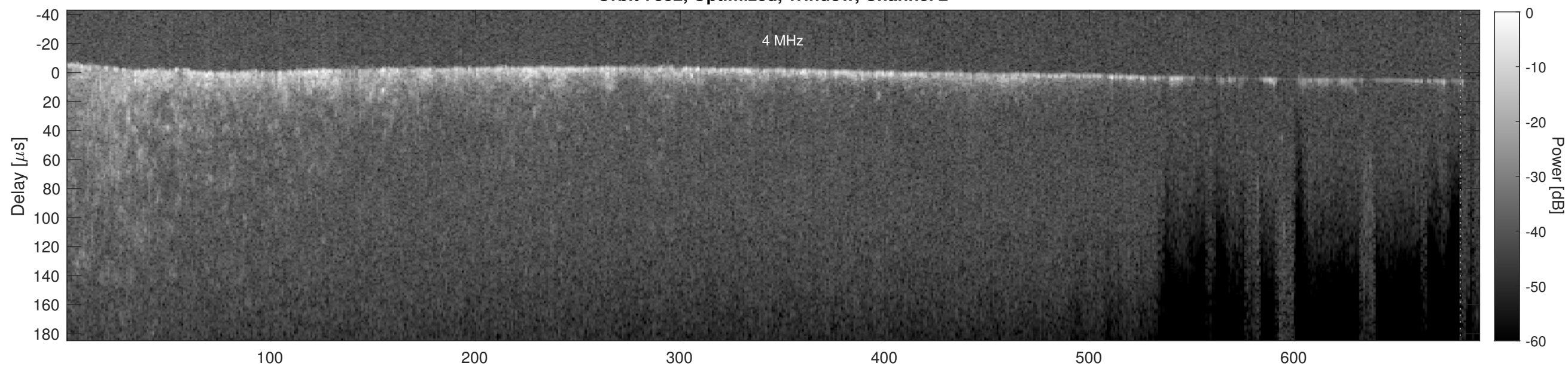
Orbit 7352, Cluttergram
