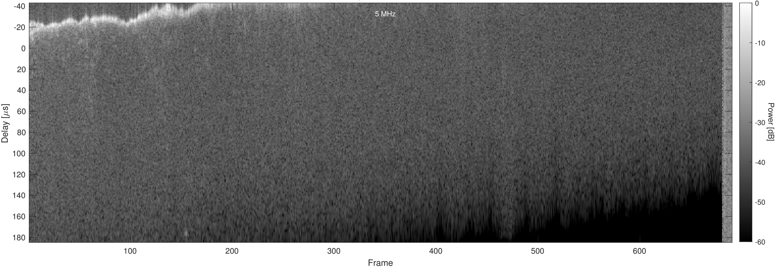
Orbit 7353, Chapman, Window, Channel 2
