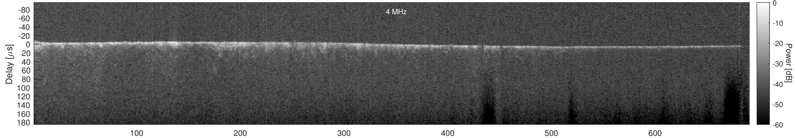
Orbit 7353, Cluttergram
