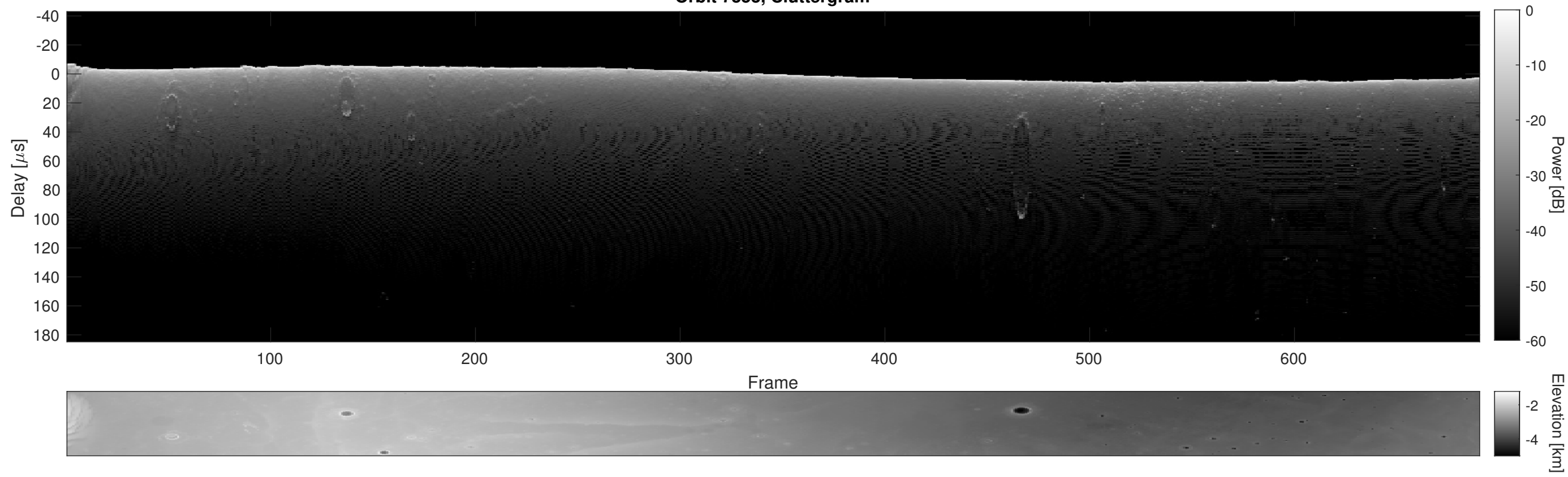
Orbit 7353, Cluttergram
