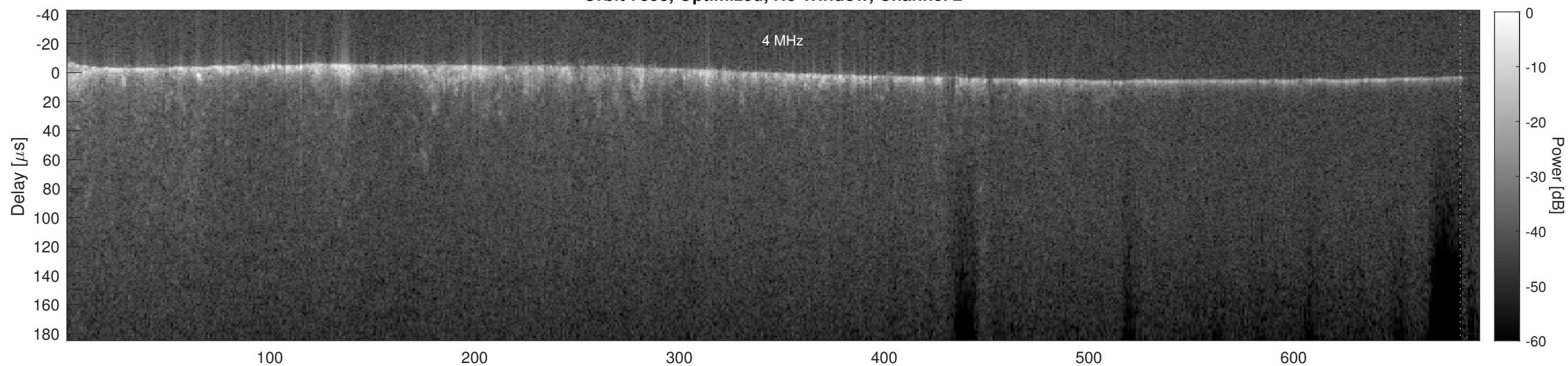
Orbit 7353, Cluttergram
