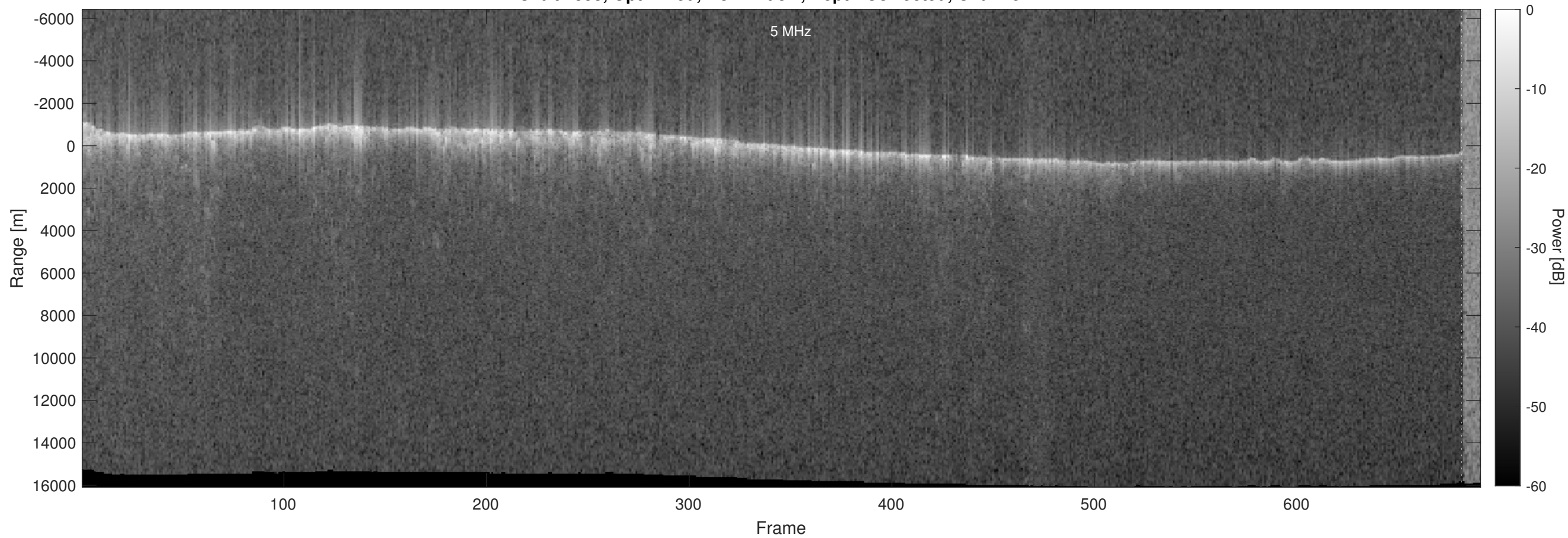
Orbit 7353, Optimized, No Window, Depth-Corrected, Channel 2
