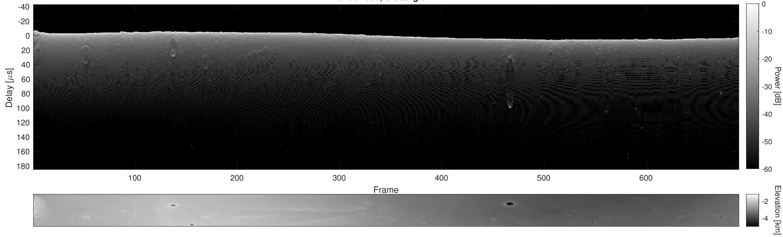
Orbit 7353, Cluttergram
