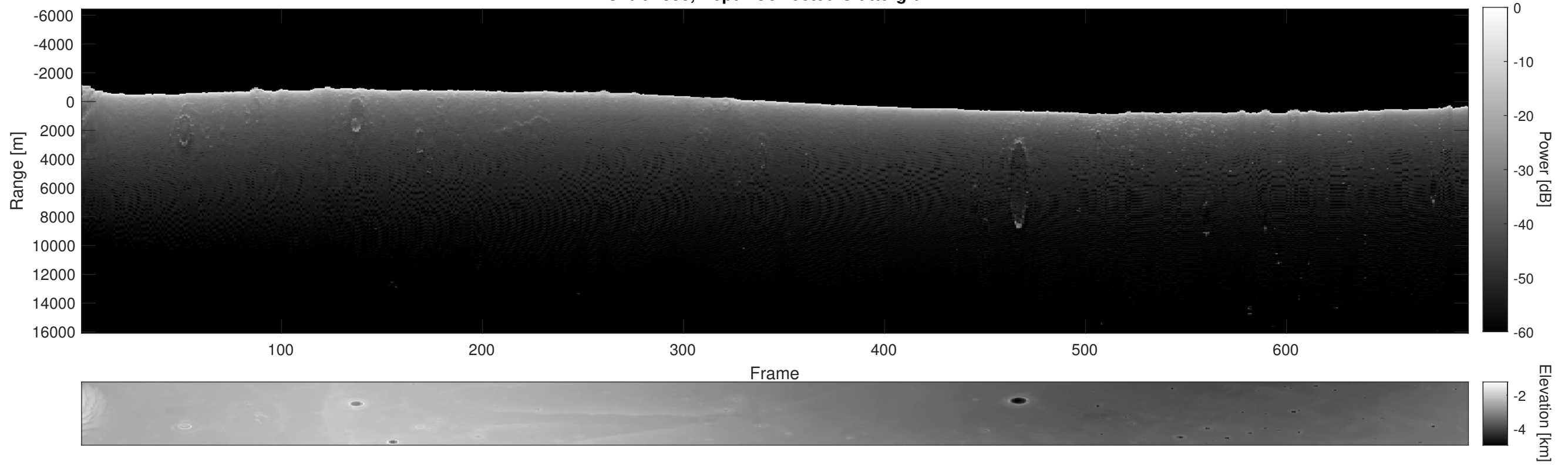
Orbit 7353, Depth-Corrected Cluttergram
