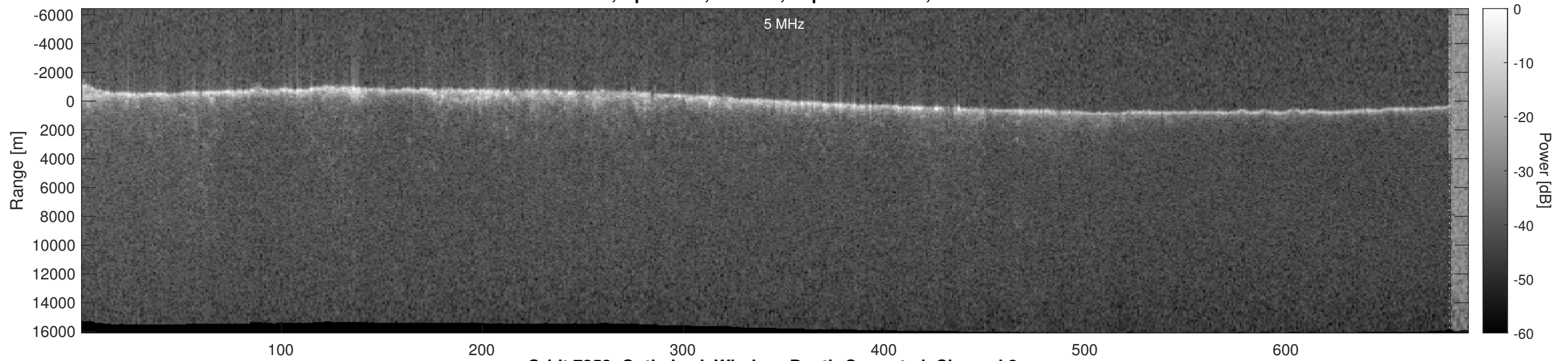
Orbit 7353, Optimized, Window, Depth-Corrected, Channel 2
