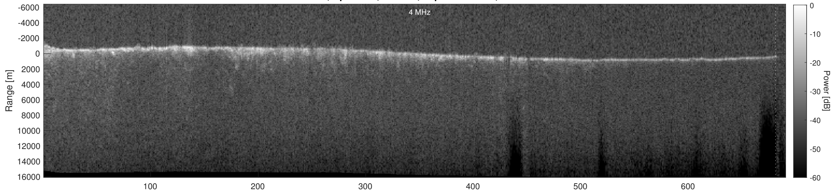
Orbit 7353, Depth-Corrected Cluttergram
