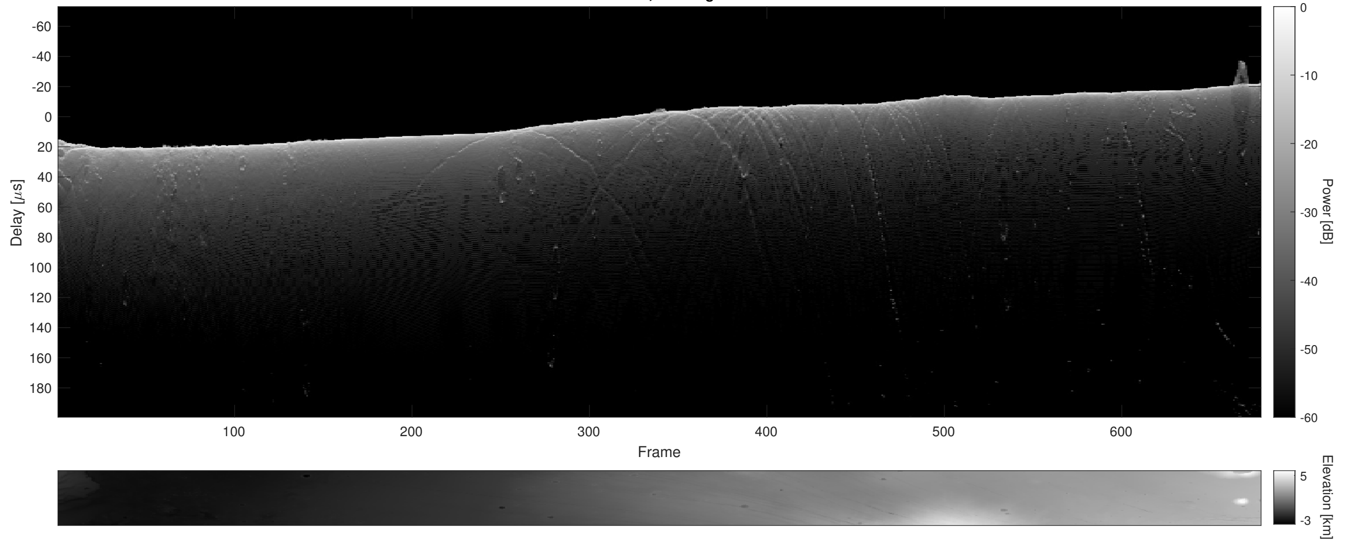
Orbit 7355, Cluttergram
