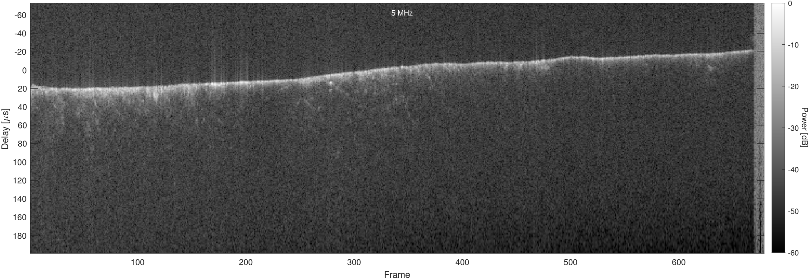
Orbit 7355, Optimized, Window, Channel 2
