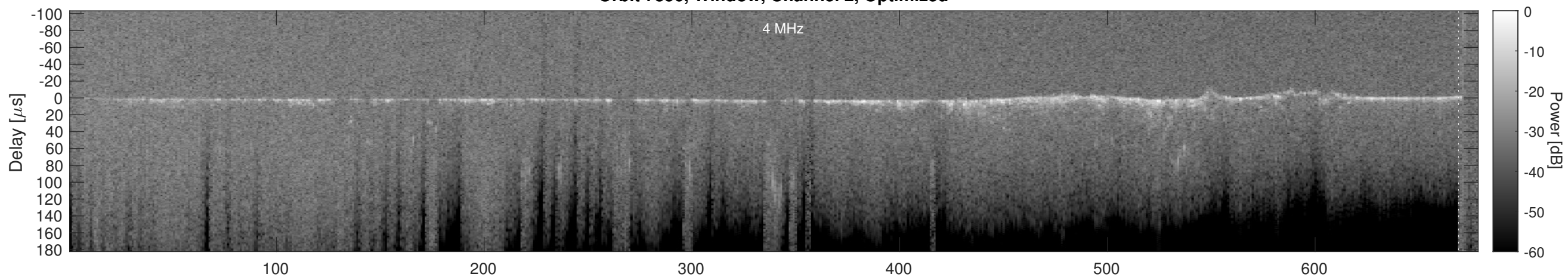
Orbit 7356, Cluttergram
