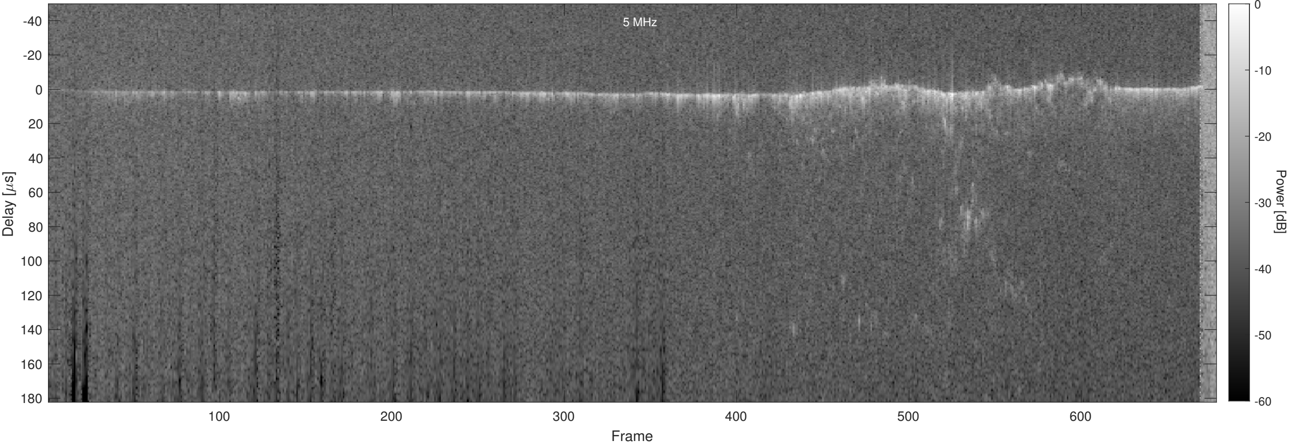
Orbit 7356, Optimized, No Window, Channel 2
