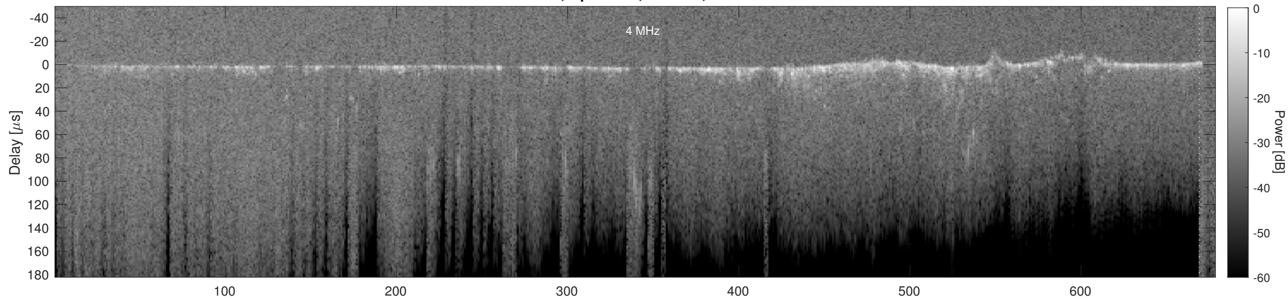
Orbit 7356, Cluttergram
