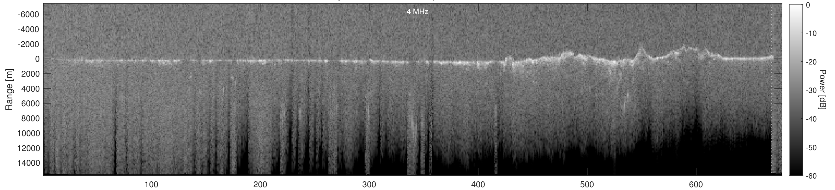
Orbit 7356, Depth-Corrected Cluttergram
