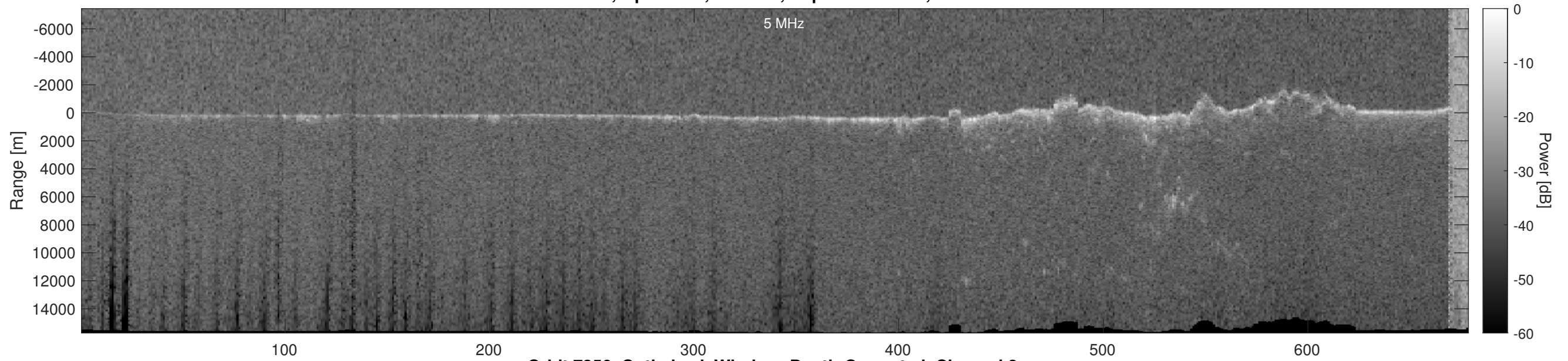
Orbit 7356, Optimized, Window, Depth-Corrected, Channel 2
