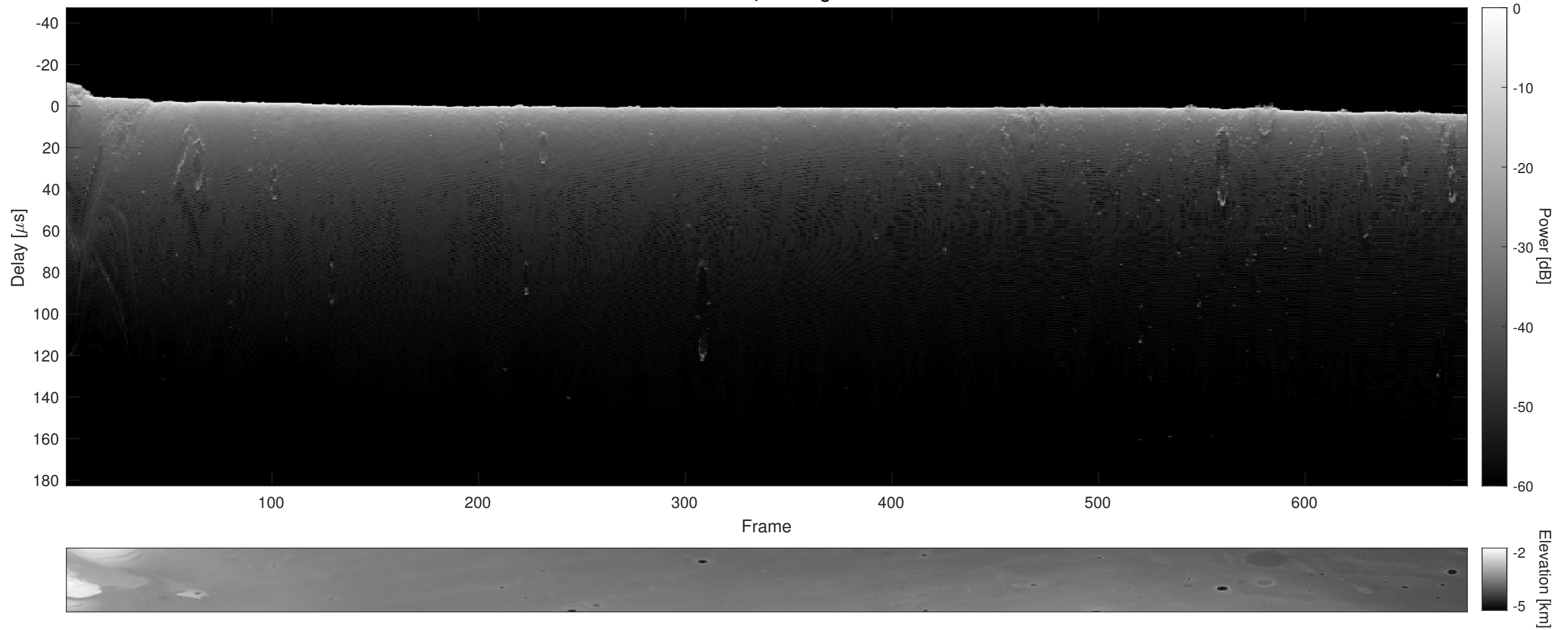
Orbit 7358, Cluttergram
