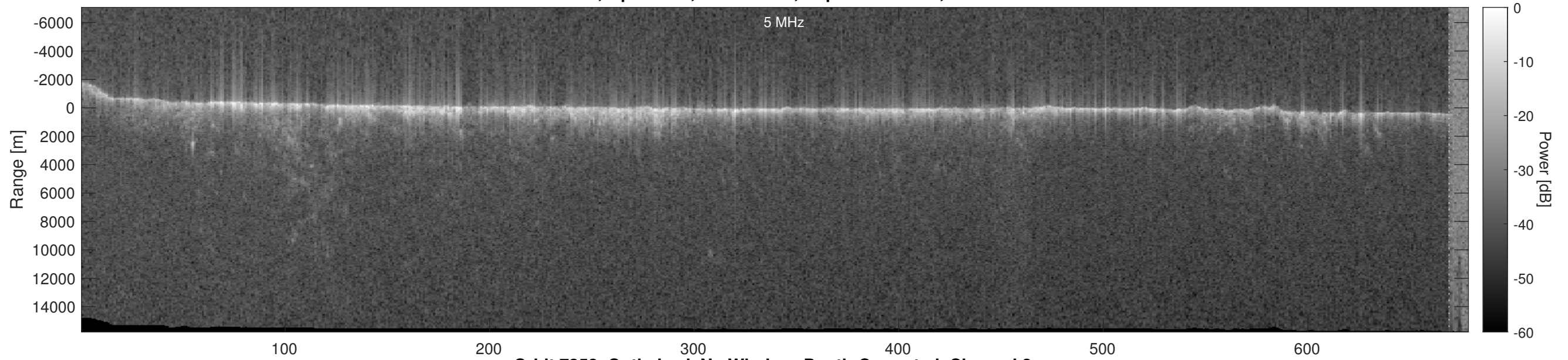
Orbit 7358, Optimized, No Window, Depth-Corrected, Channel 2
