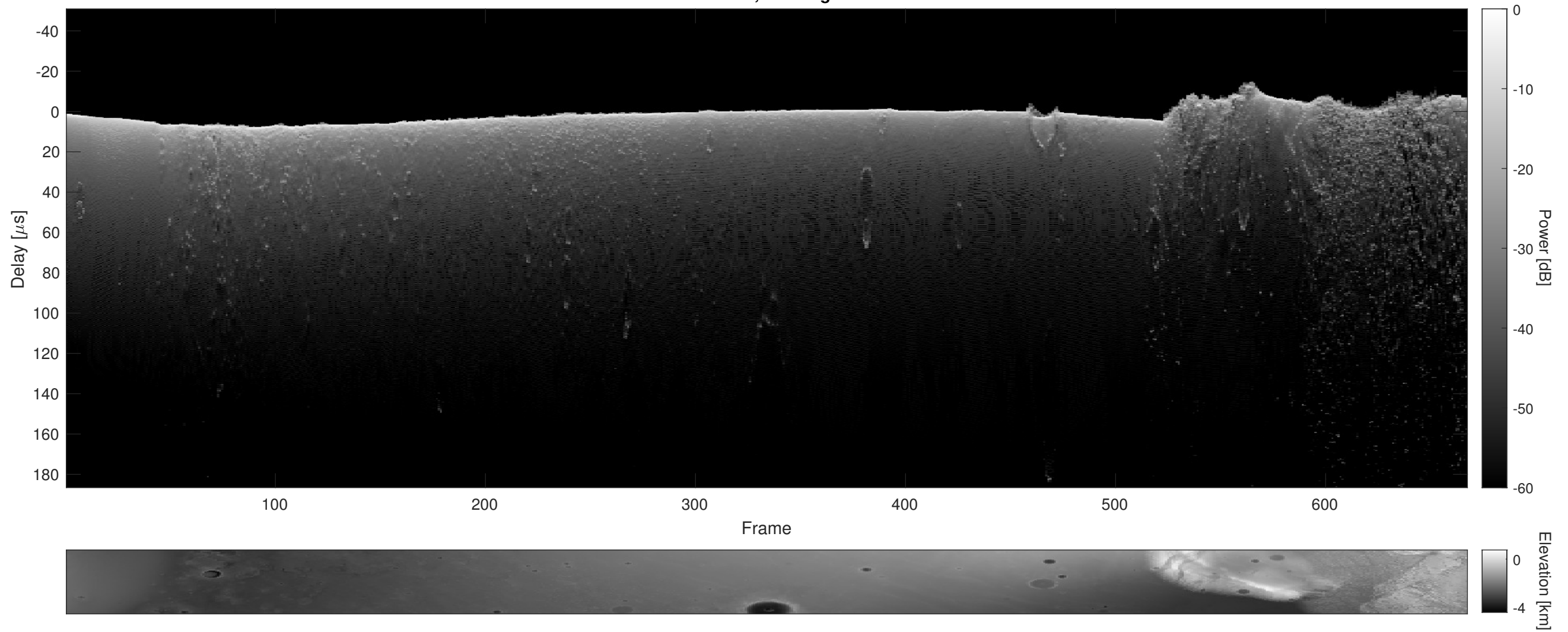
Orbit 7359, Cluttergram
