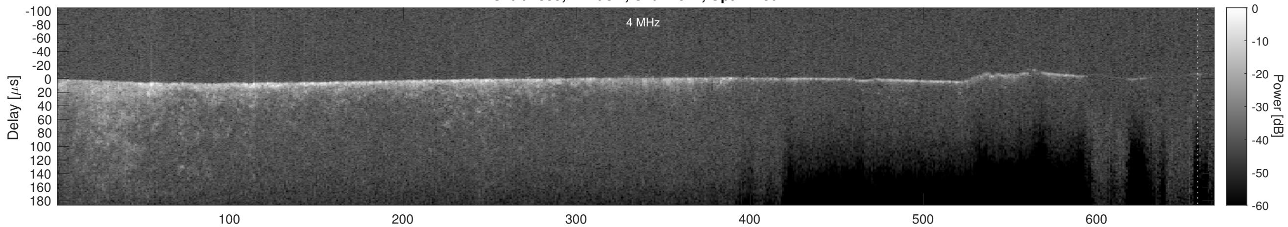
Orbit 7359, Cluttergram
