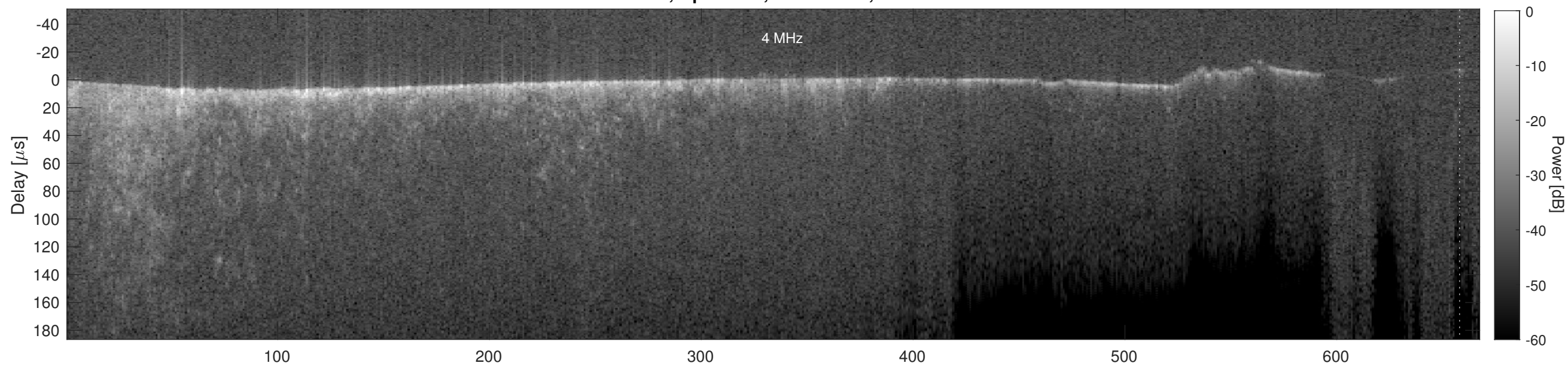
Orbit 7359, Cluttergram
