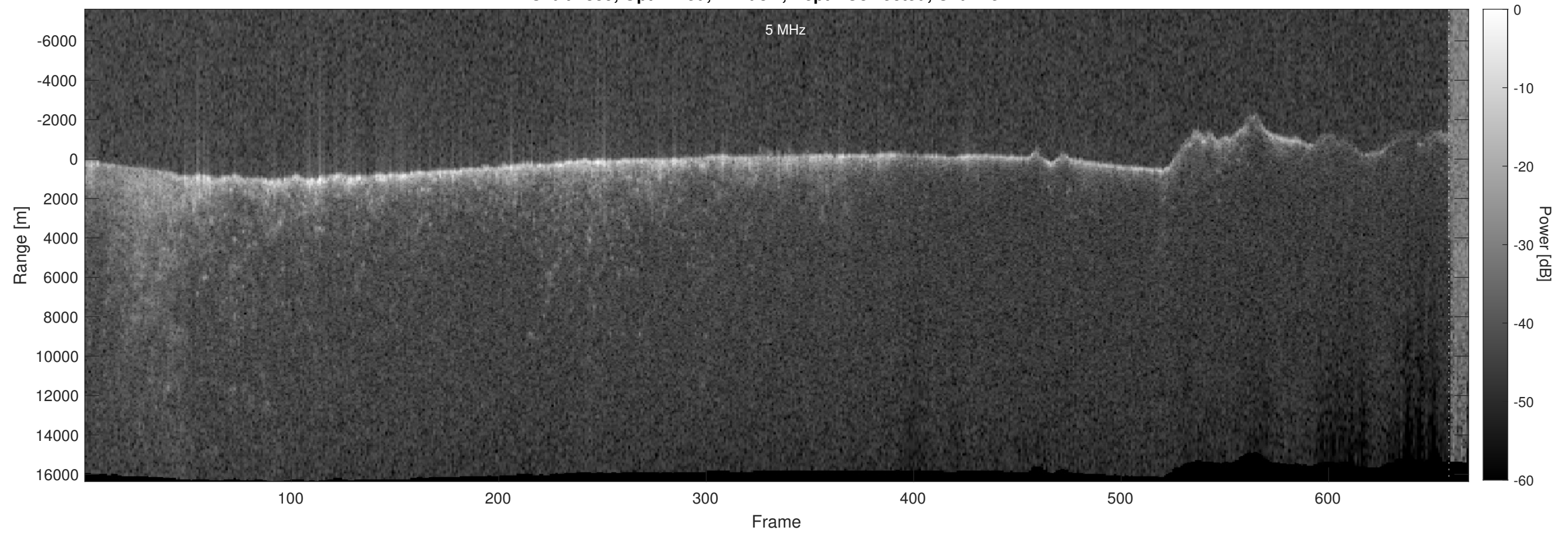
Orbit 7359, Optimized, Window, Depth-Corrected, Channel 2
