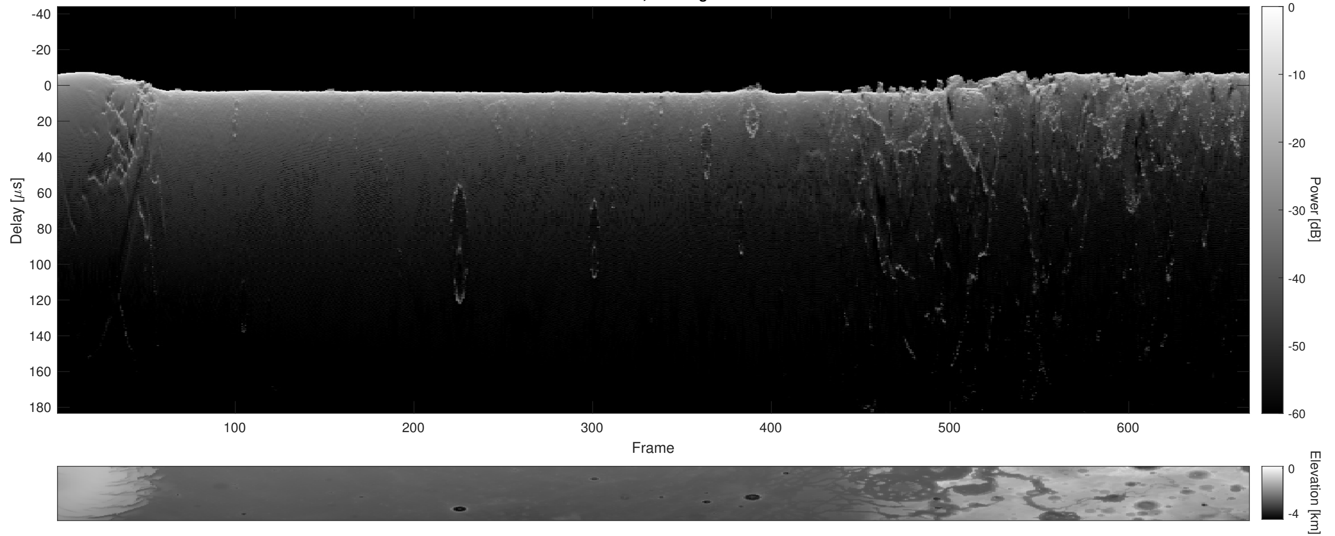
Orbit 7361, Cluttergram
