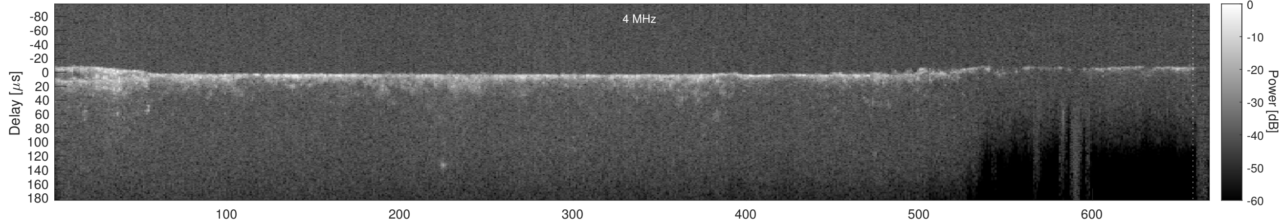
Orbit 7361, Cluttergram
