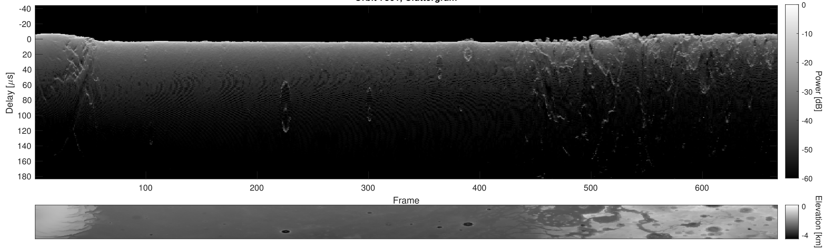
Orbit 7361, Cluttergram
