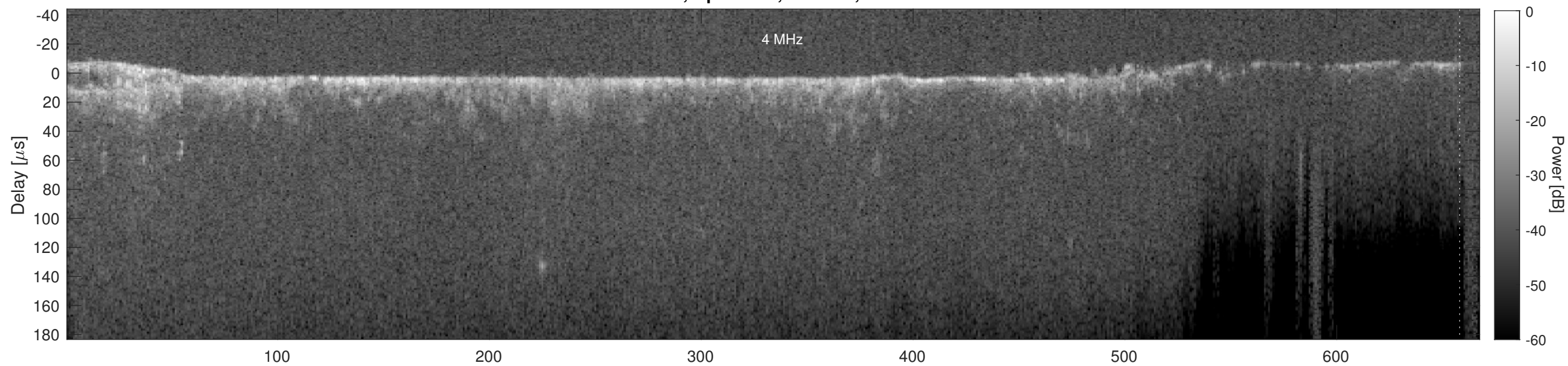
Orbit 7361, Cluttergram
